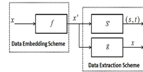
Figure 3: The data Embedding and Extraction procedure
